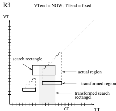
Figure 6: Search Specifics for Tree R3
