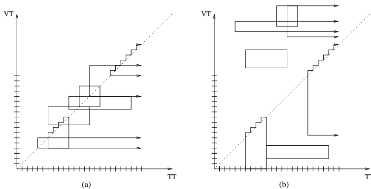
Figure 7: Influence of Dev on Data Distribution in the GR-tree; (a) Small and (b) Large Dev
