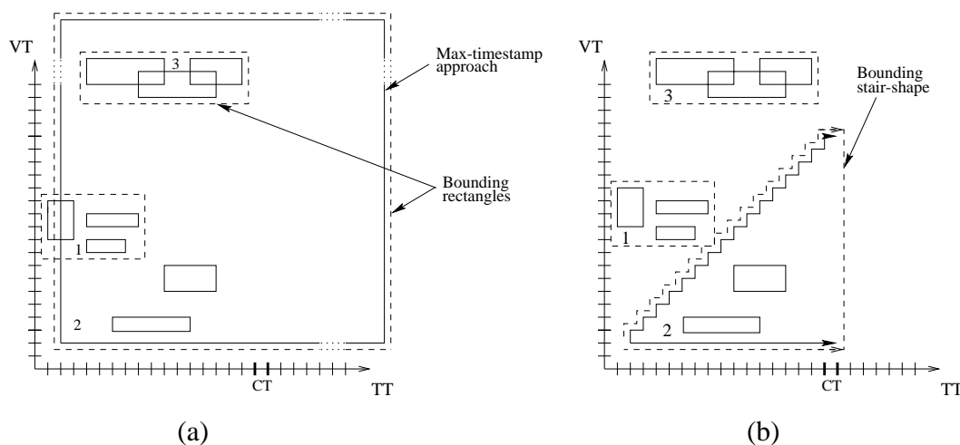
Figure 3: Indexing Growing Bitemporal Regions (a) Using Maximum-Timestamp Values and (b) Using the GR-Tree
