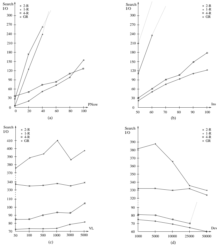
Figure 8: Search Performance for Average Workload Parameters, but (a) Varying PNow , (b) Ins , (c) VL , and (d) Dev
