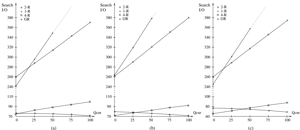
Figure 10: Search Performance for Average Workload Parameters, but Varying Q_{cur} for (a) Range Queries, (b) Timeslice Queries, and (c) Point Queries
