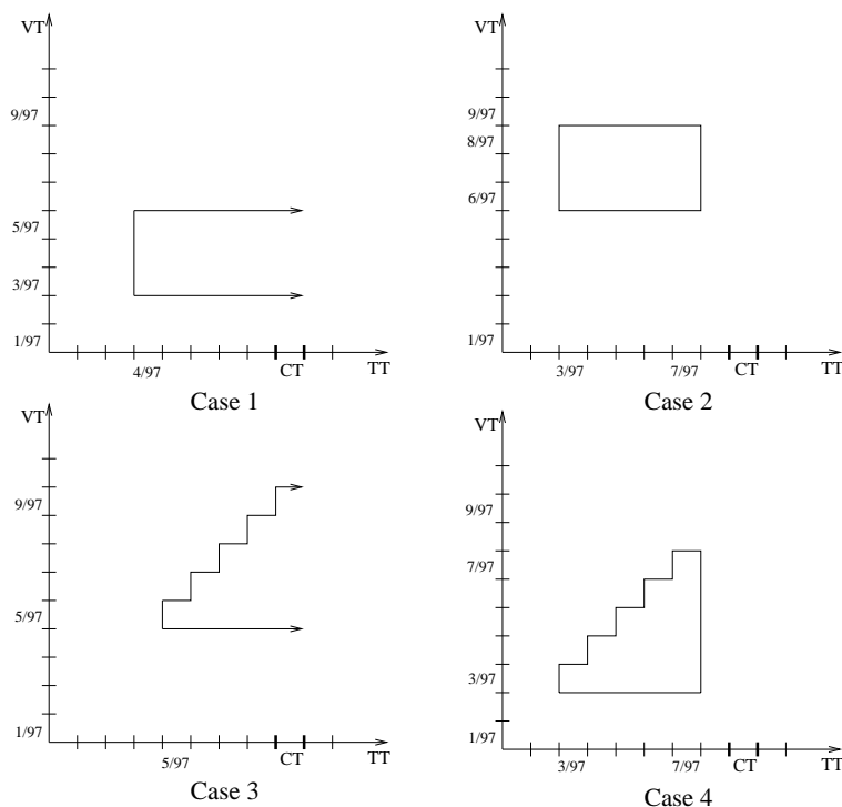
Figure 1: Bitemporal Regions
