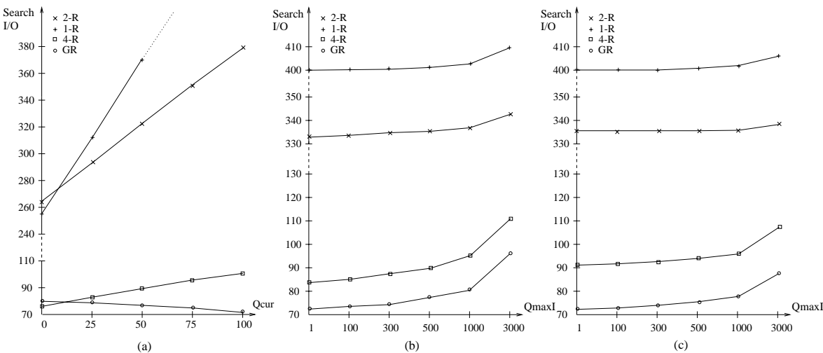
Figure 11: Search Performance for Average Workload Parameters, but Varying Q_{cur} for (a) Mixed Queries and Varying Q_{maxI} for (b) Range Queries and (c) Timeslice Queries
